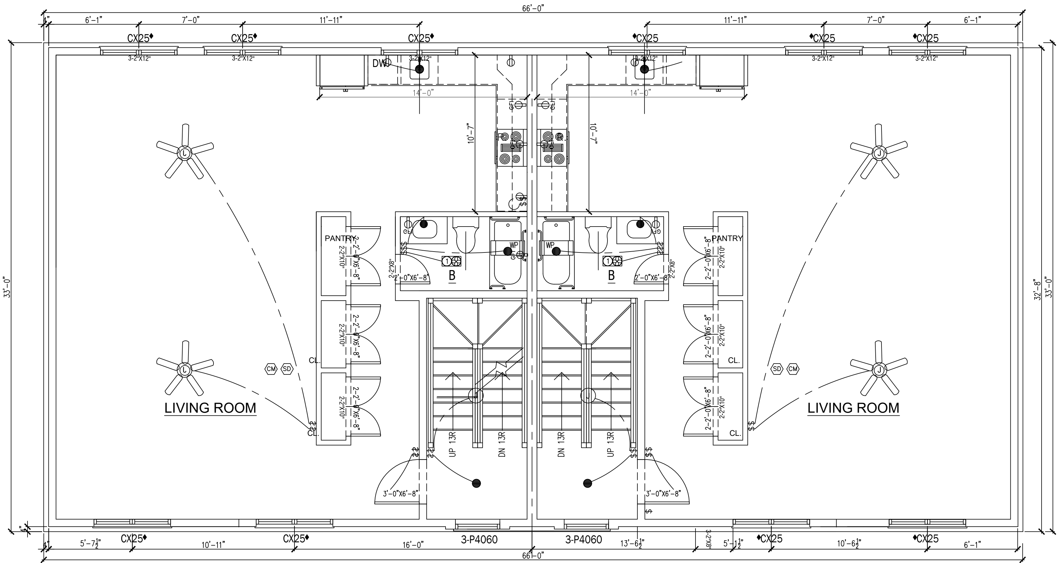
2 FIRST FLOOR PLAN
