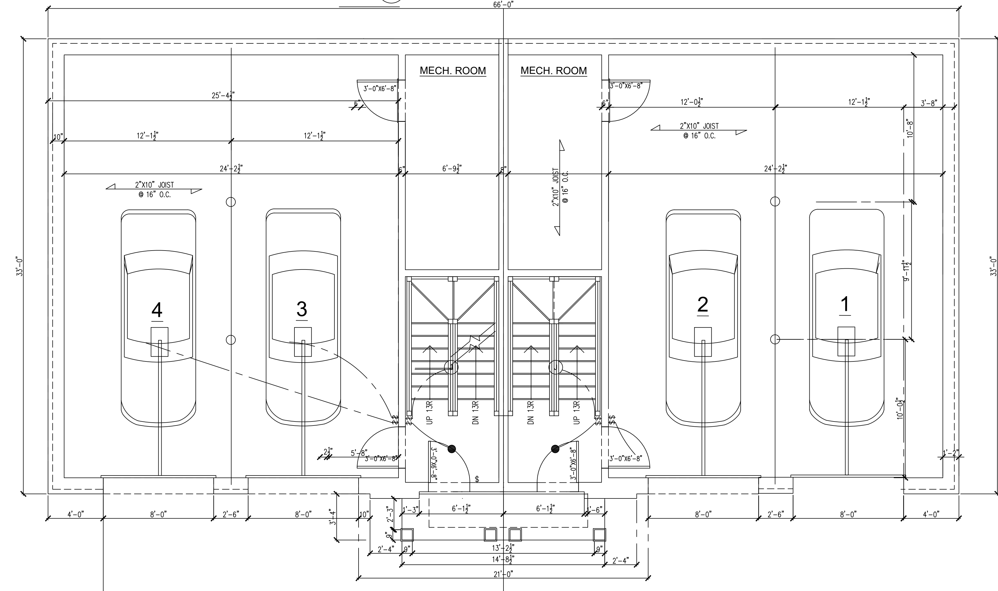
1 CELLAR PLAN
