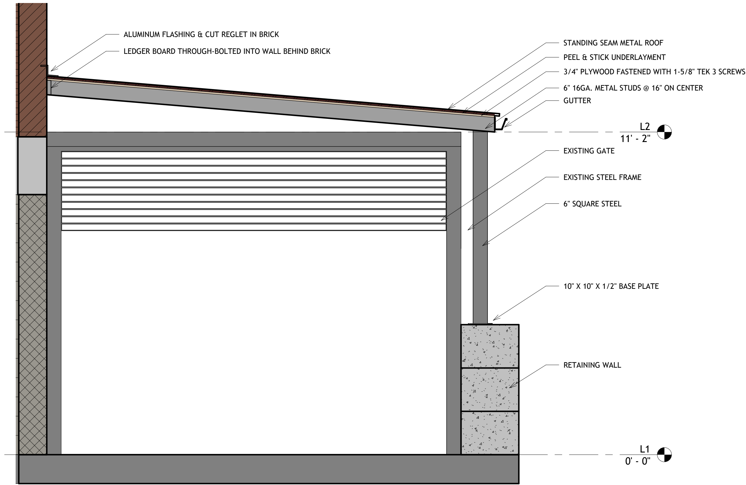
① East View 1/2" = 1'-0"
