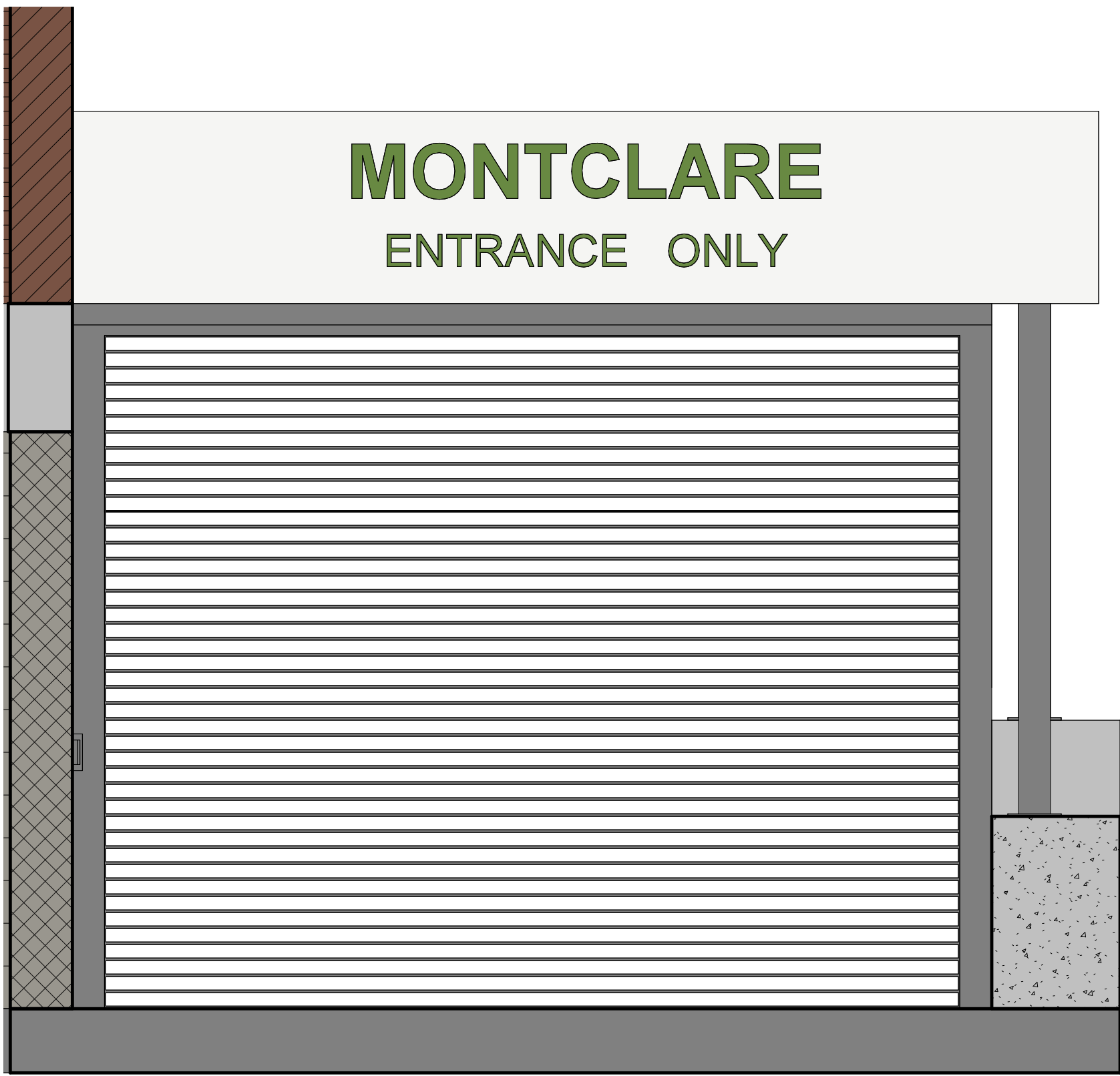
② East View End Result 1/2" = 1'-0"
